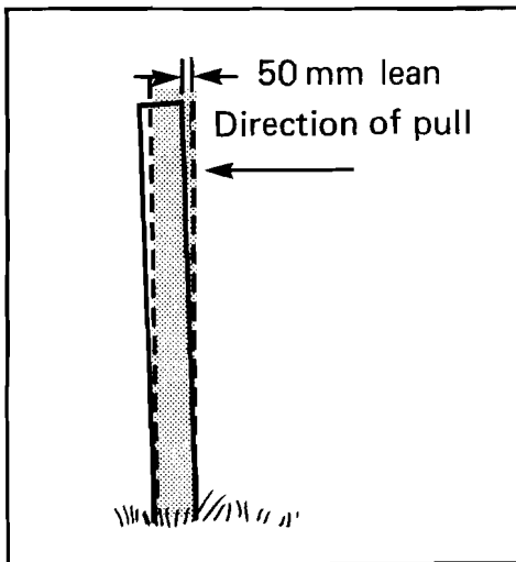
Fig. 18 Proper placement of end posts.
