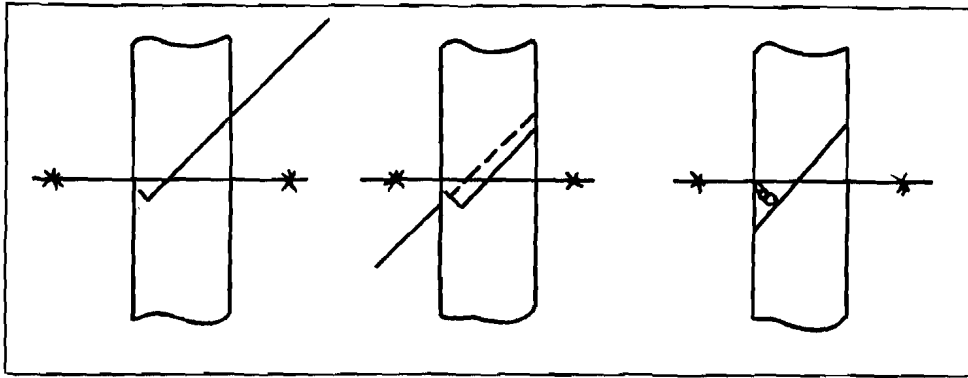
Fig. 41 Single wrap for dropper attachment.
