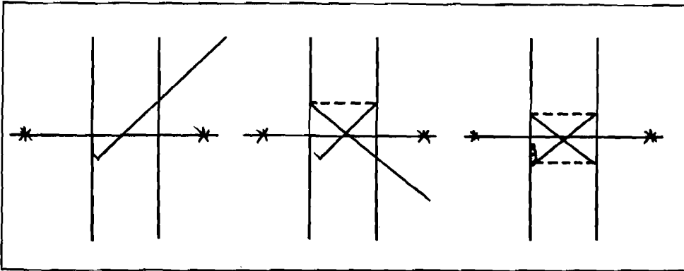
Fig. 42 Figure eight wrap for dropper attachment.
