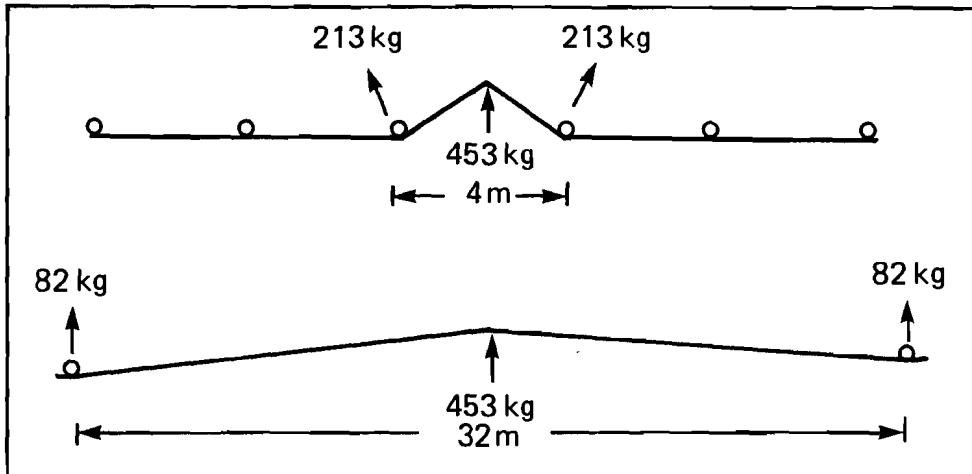
Fig. 2 Effect of post spacing on lateral loads applied to a fence.
