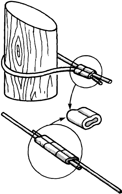
Fig. 8 Oval compression sleeves.
