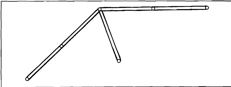
Fig. 32 Double brace assembly for shallow corner in soft or boggy soils.
