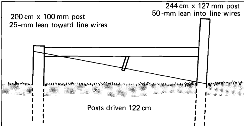
Fig. 31 Medium corner brace assembly (Fig. 30) showing construction.
