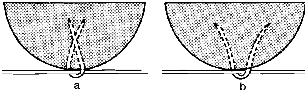
Fig. 36 Staples driven (a) incorrectly and (b) correctly.
