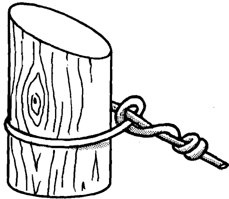
Fig. 7 Knot for tying off high-tensile wire.
