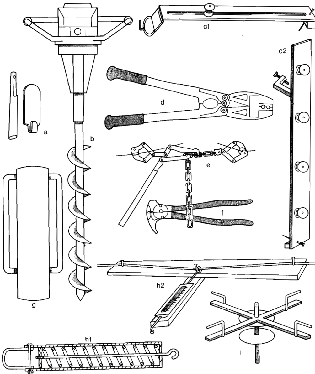
Fig. 13 Special fencing tools.
