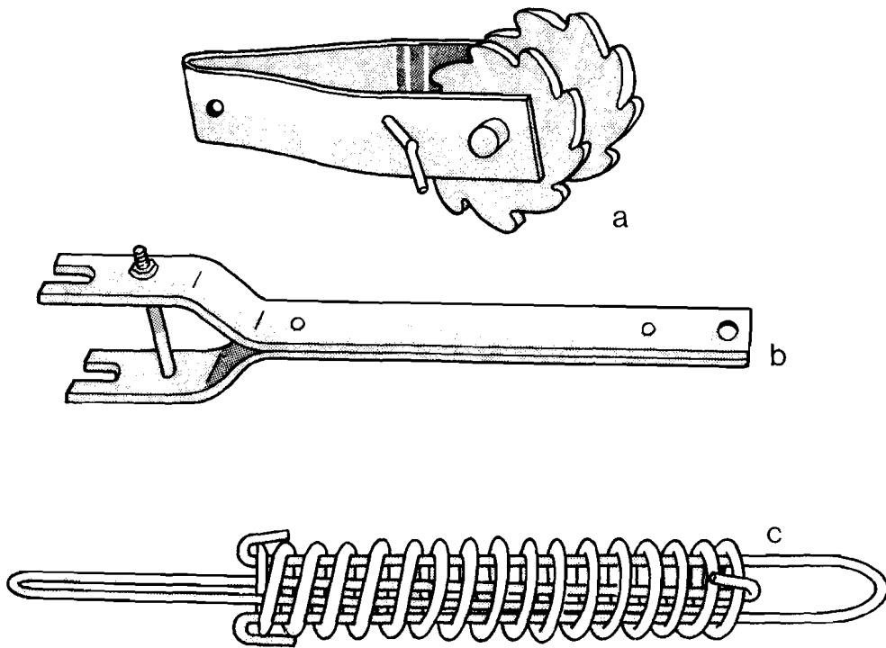
Fig. 12 (a) In-line wire strainer, (b) handle, and (c) tension-indicator spring.
