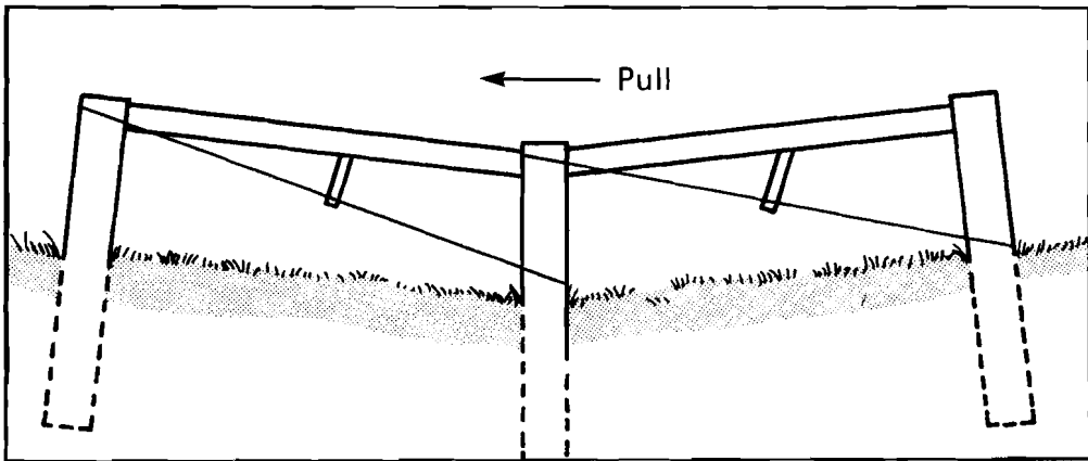
Fig. 29 Double-span dip assembly.
