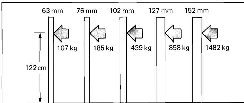
Fig. 4 Average breaking strengths for pressure-treated pine posts with loads steadily applied.
