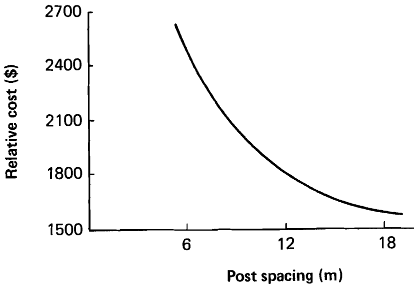
Fig. 1 Post spacing versus fence costs.
