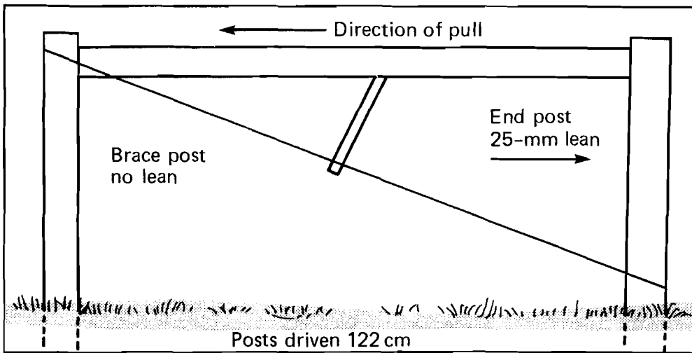
Fig. 26 Single-span brace assembly.
