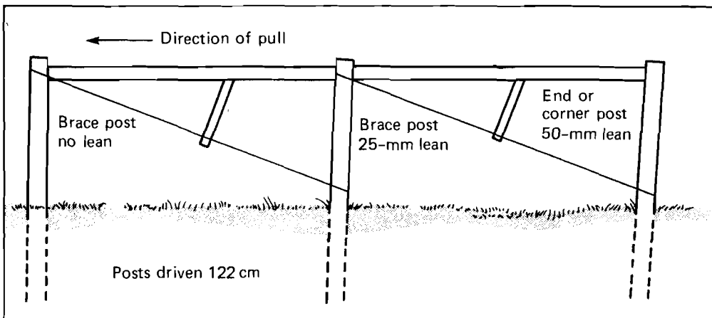
Fig. 27 Double-span brace assembly.
