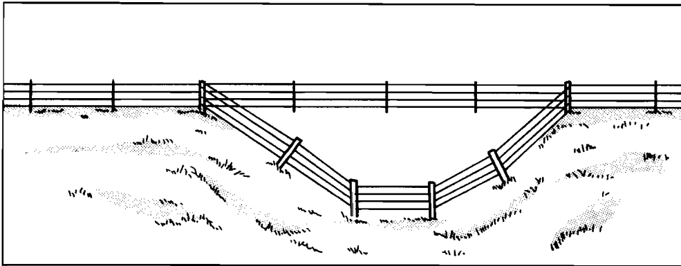
Fig. 21 Bridging a narrow gully with high-tension fence.
