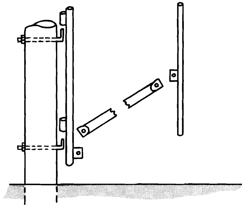
Fig. 45 Hinged wire gate.
