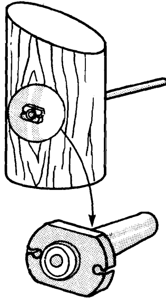
Fig. 9 Wirevise for high-tensile wire.
