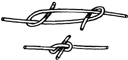
Fig. 10 Figure-eight knot for splicing high-tensile wire.
