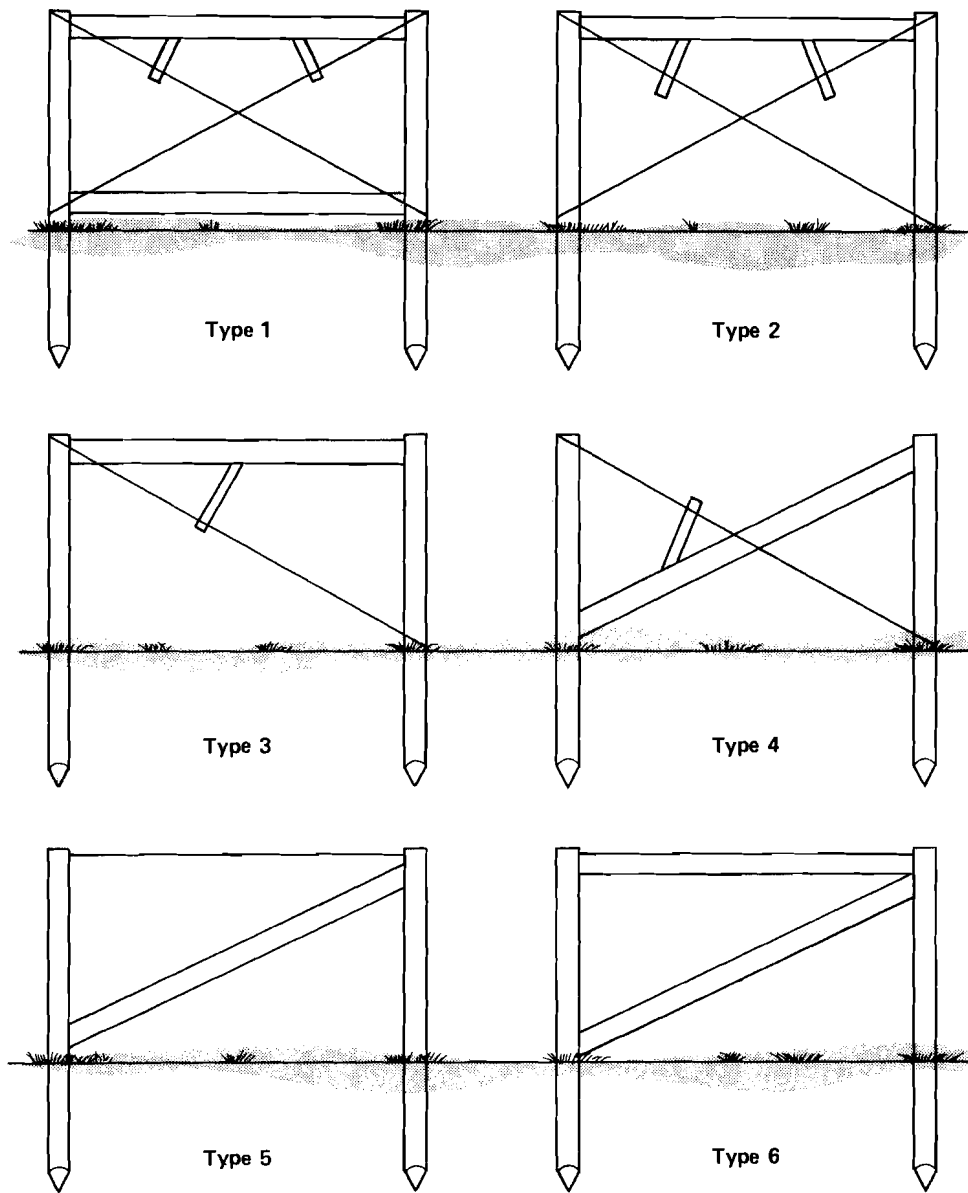
Fig. 3 Types of brace assemblies tested.
