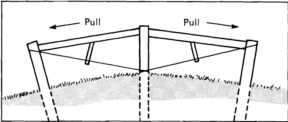
Fig. 28 Double brace assembly for rise posts.
