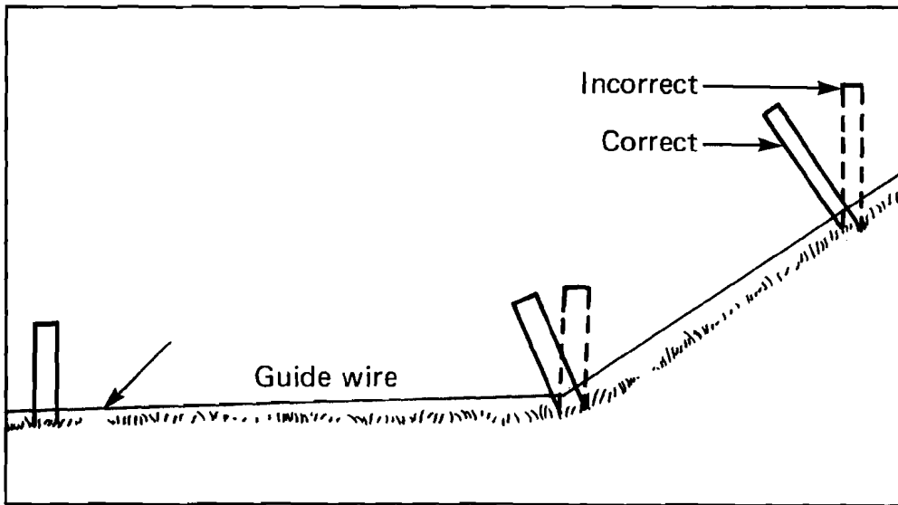
Fig. 34 Vertical placement of line posts.
