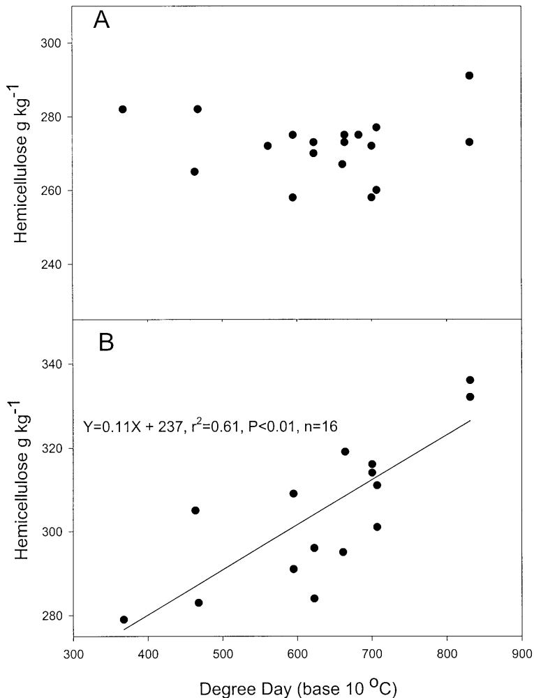
Fig. 1. Mean hemicellulose concentration as influenced by accumulated degree day (base 10°C) at each site-year for: (A) cool-season grass mean at each site-year ( n = 18 ) and (B) warm-season grass mean at each site-year ( n = 16 ).
