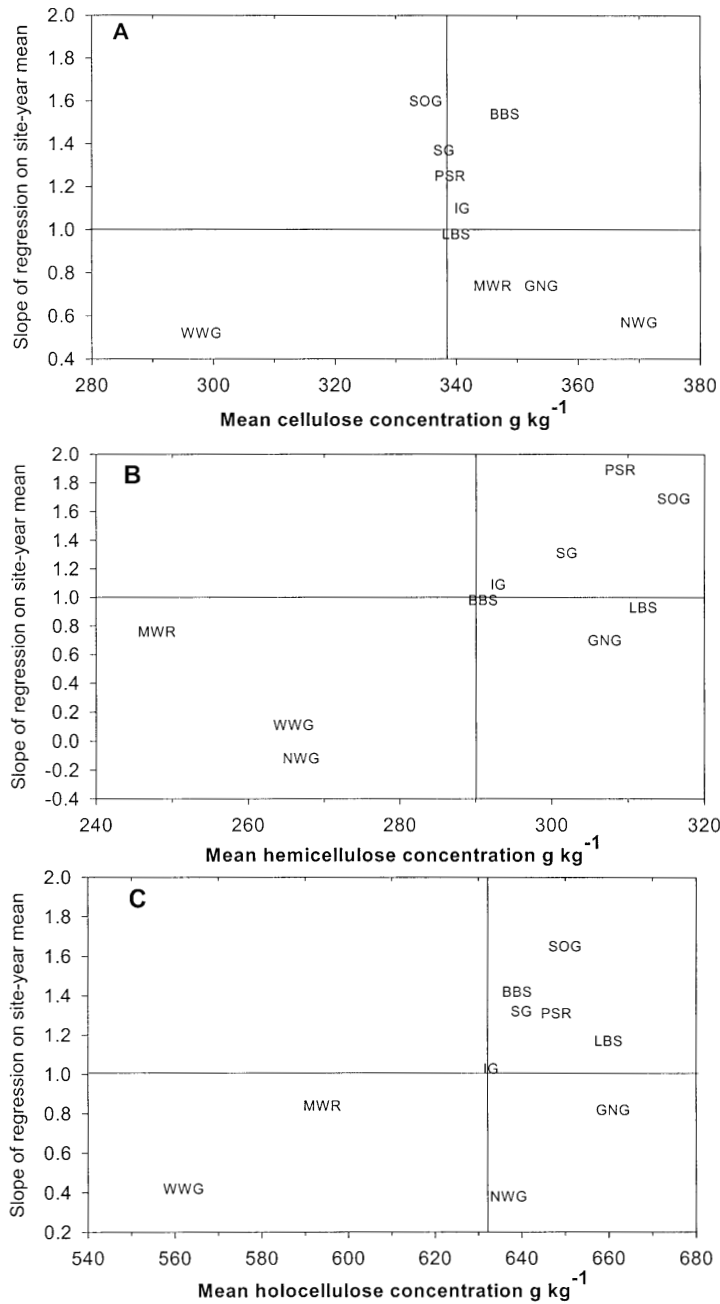
Fig. 2. Slope of regression of cellulose (A), hemicellulose (B) and holocellulose (C) concentration of each species on site mean relative to overall species mean. Species abbreviations used as symbols are: BBS, big bluestem; GNG, green needlegrass; IG, indiagrass; LBS, little bluestem; MWR, mammoth wildrye; NWG, northern wheatgrass; PSR, prairie sandreed; SG, switchgrass; SOG, sideoats grama; and WWG, western wheatgrass. Reference lines are drawn at slope 1.0 and overall mean concentration.
