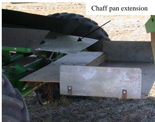
Photo 11: An extension plate ensures the chaff falls behind the hinge point.
